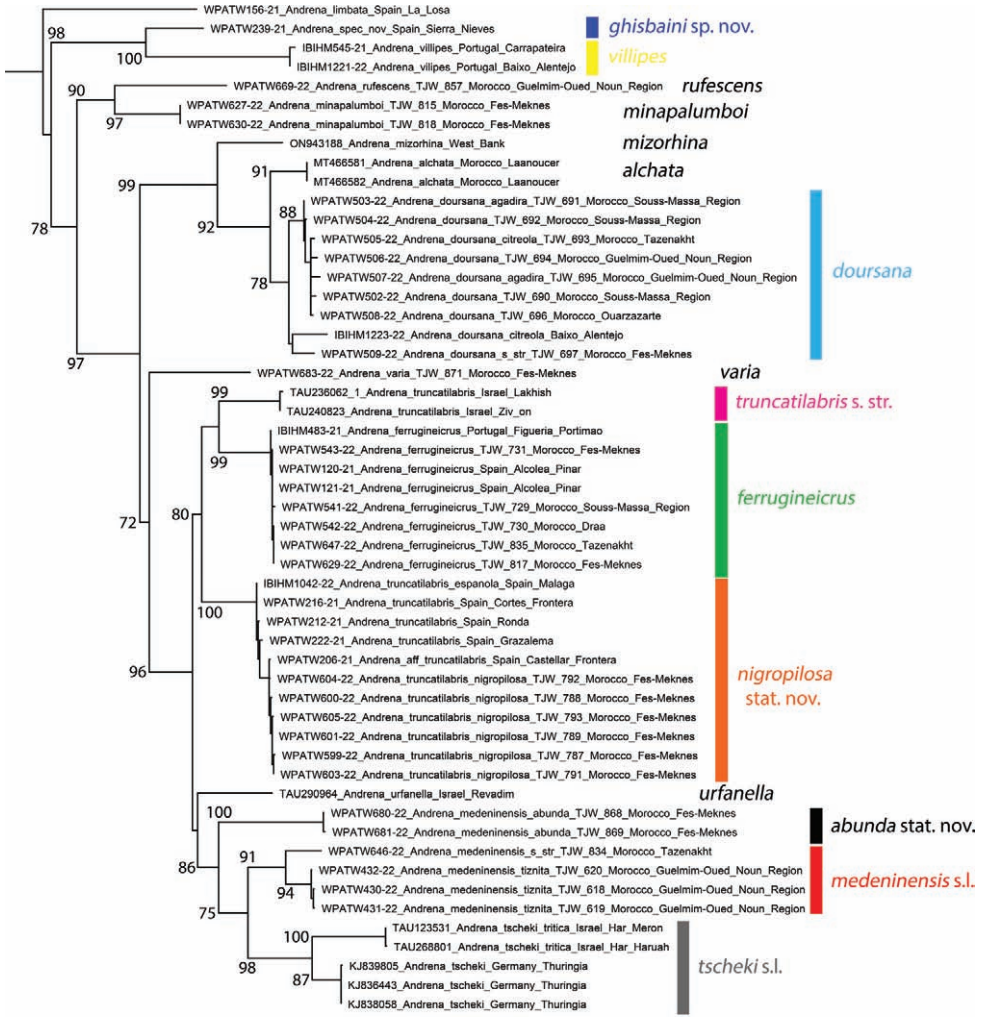
Figure 29. Phylogenetic tree (maximum likelihood) of Andrena subgenus Truncandrena Warncke, 1968 based on the mitochondrial COI gene. Andrena (Limbandrena) limbata Eversmann, 1852 is used as an outgroup. Numbers adjacent to branches represent bootstrap support (values of <75 are omitted).
